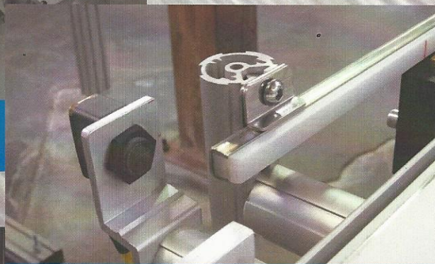
THRU BEAM SENSOR & GUIDE RAIL MOUNT
