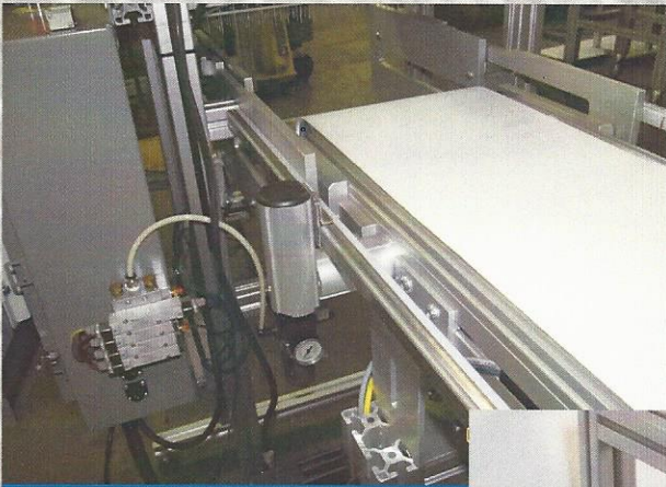
CONVEYOR GUIDE ROLLER CONVEYOR
