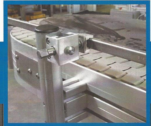
CONVEYOR GUIDE RAIL MOUNTS
